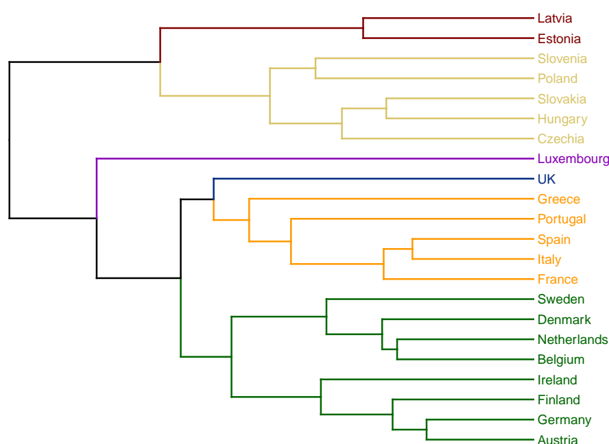
Cluster Dendrogram
