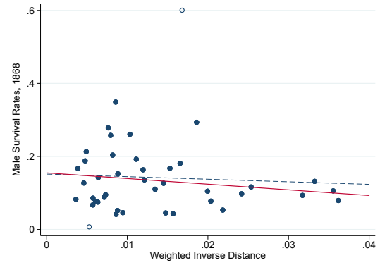
(b) MSR^{i,1,3}
