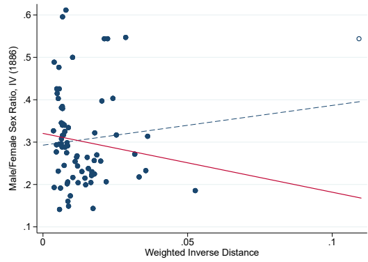
(a) MFSR^{i,1,2}
