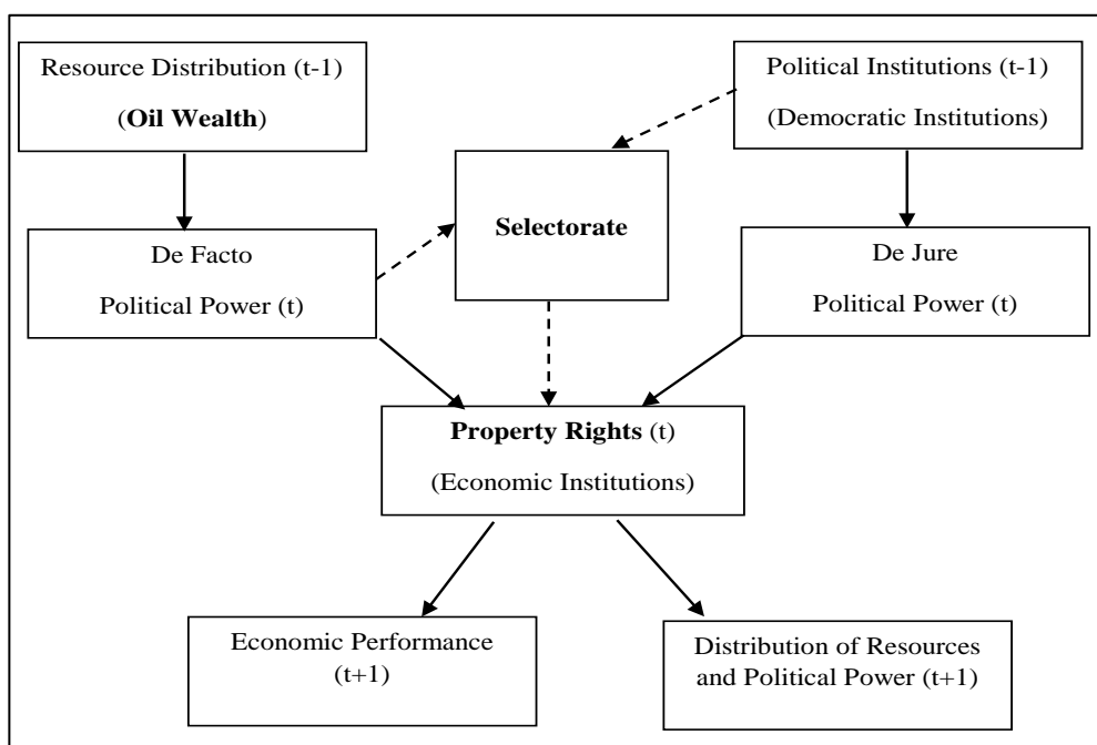
Figure 1: Theoretical Framework
