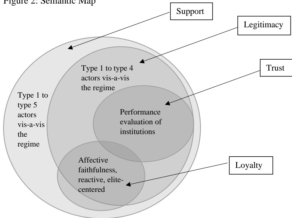
Figure 2: Semantic Map
