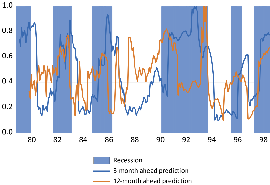
Figure 3: Predicted recession probabilities for h = 3 and h = 12 months ahead
