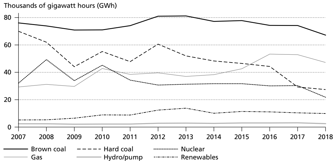
Figure 2 RWE electricity generation mix
