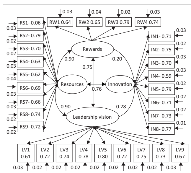
FIGURE 4: The structural equation model.
