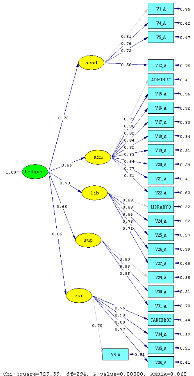
Figure 2: Higher order factor
