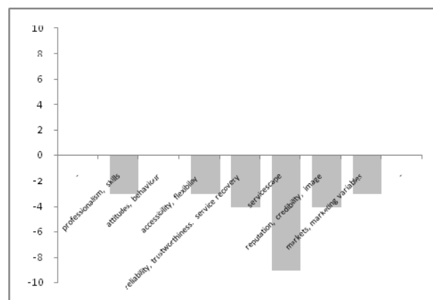
Figure 5: The underlying drivers of consumption in Factor 2
