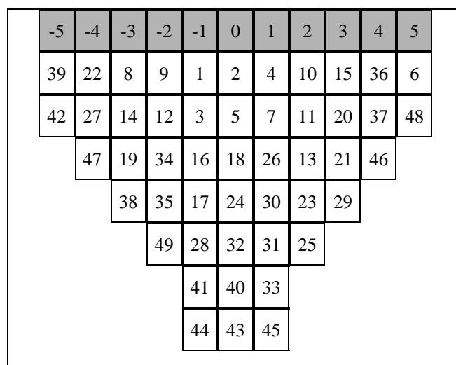
Figure 3: The visual presentation of individual factors
