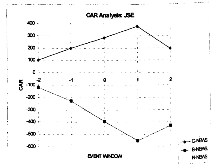
Figure 3 CAR plot for the JSE
