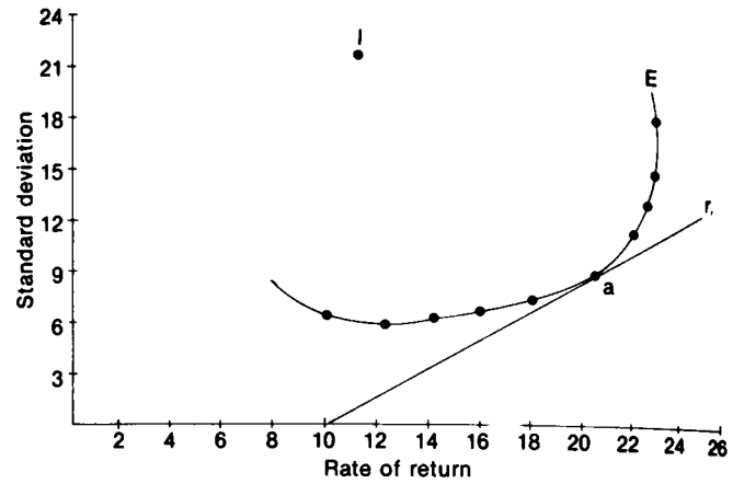
Figure 3 Efficient portfolios available from international diversification (33% limit to investment in specific country)
