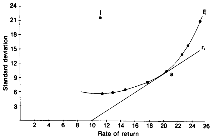
Figure 1 Efficient portfolios available from international diversification (no limit to investment in specific country)
