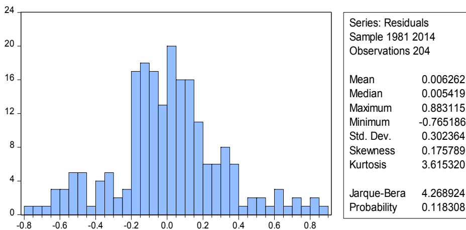
Figure 2: Normality Test
