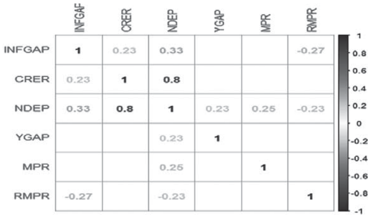
Figure 1: Linear correlation matrix for the macro-variables at time-domain
