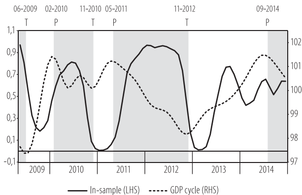
Figure 2: Estimated probabilities and the GDP cycle
