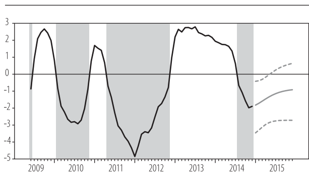
Figure 4: Posterior mean of latent variable and its 12-months-ahead forecast (shaded areas indicate recession dates)
