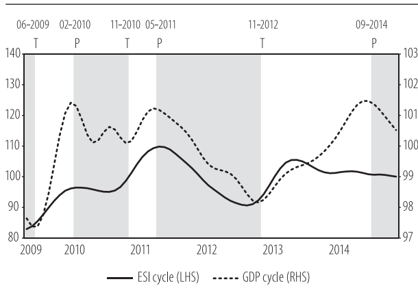
Figure 1: Cyclical components of ESI and GDP
