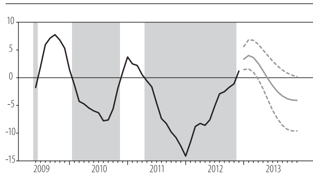
Figure 3: Posterior mean of latent variable and its 12-months-ahead forecast (shaded areas indicate recession dates)
