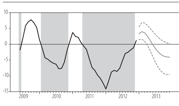
Figure 3: Posterior mean of latent variable and its 12-months-ahead forecast (shaded areas indicate recession dates)
