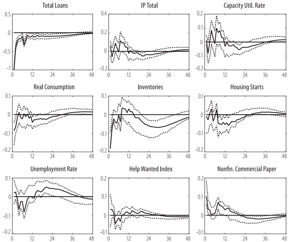
Figure 2: Impulse response functions of economic activity variables to a negative shock of the total bank loans, generated from the FAVAR model. The dotted lines represent a 95% confidence band around the impulse response functions.
