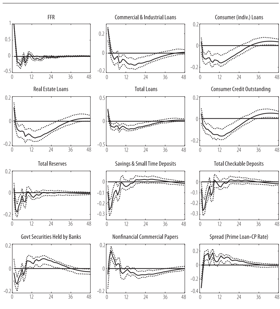
Figure 1: Impulse response functions of bank portfolio variables to a contractionary monetary policy shock (measured by the FFR), generated from the FAVAR model. The dotted lines represent a 95% confidence band around the impulse response functions.
