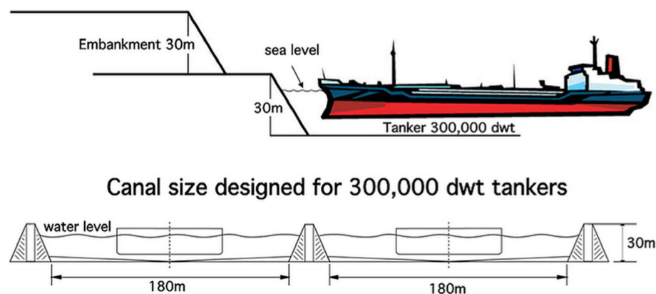
Fig. 2 Proposed design parameters of canal (Kra Canal International Forum 2014)
