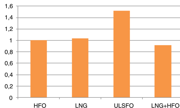
Fig. 11 OPEX differences with different fuels and alternatives (LNG = using LNG all the time whilst LNG + HFO = HFO is used outside ECAs). Relative differences: 1 = costs running on HFO
