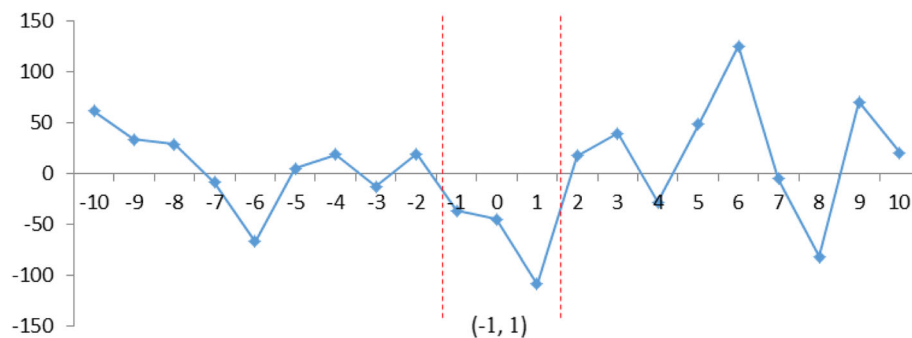
Fig. 3 Average CAR in the(-10,10)window
