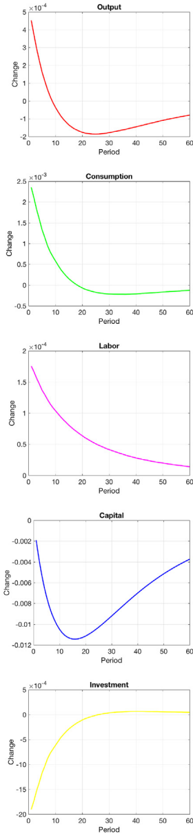
Fig. A.1. Impulse-Response Functions of Stochastic \sigma Model to Risk Aversion Shock.
