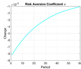
Fig. A.2. Impulse-Response Functions of Risk Aversion Coefficient \sigma to TFP Shock.
