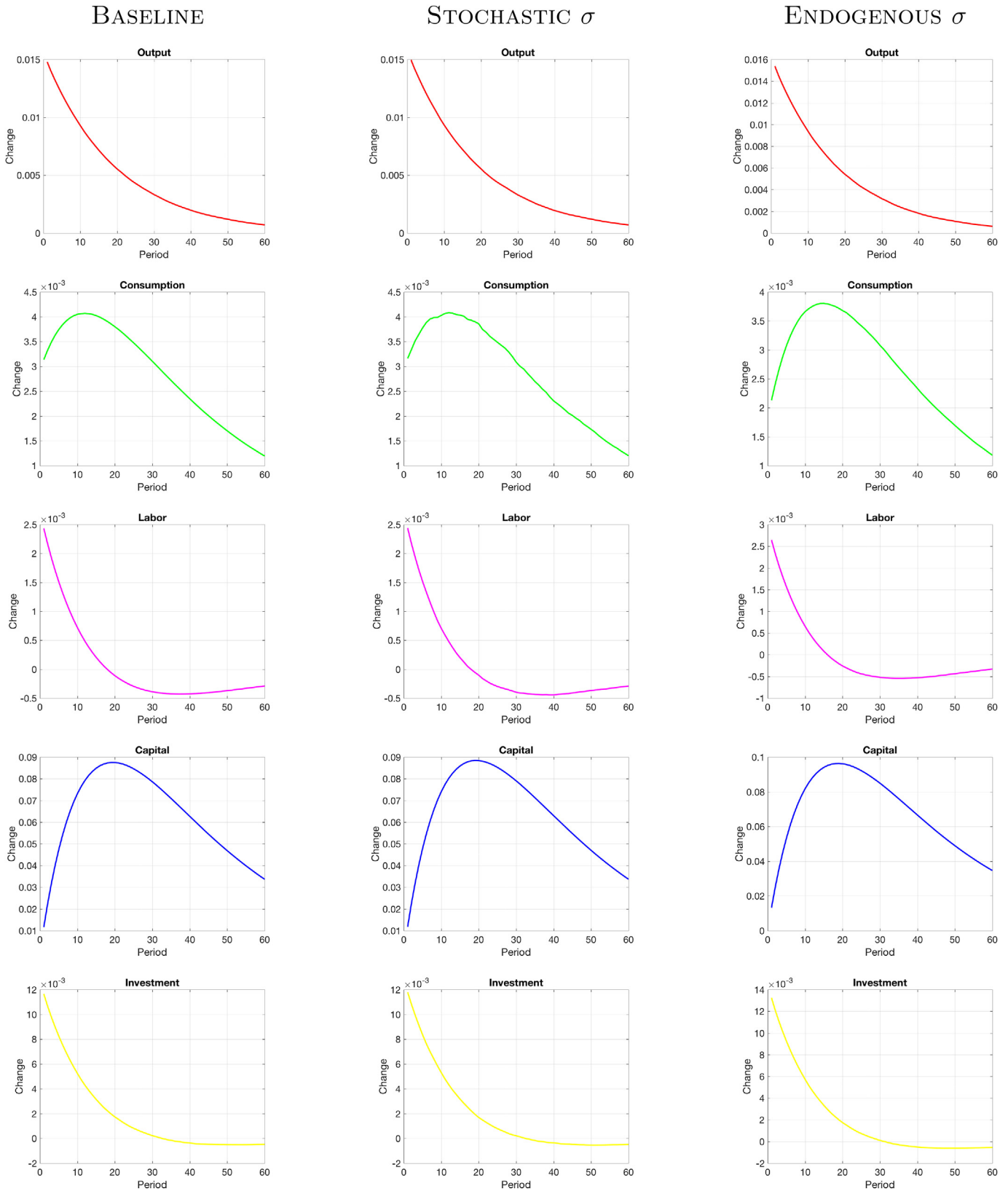
Fig. 2. Impulse-Response Functions with Hansen-Rogerson Parameter Set ( \nu = 0 ).
