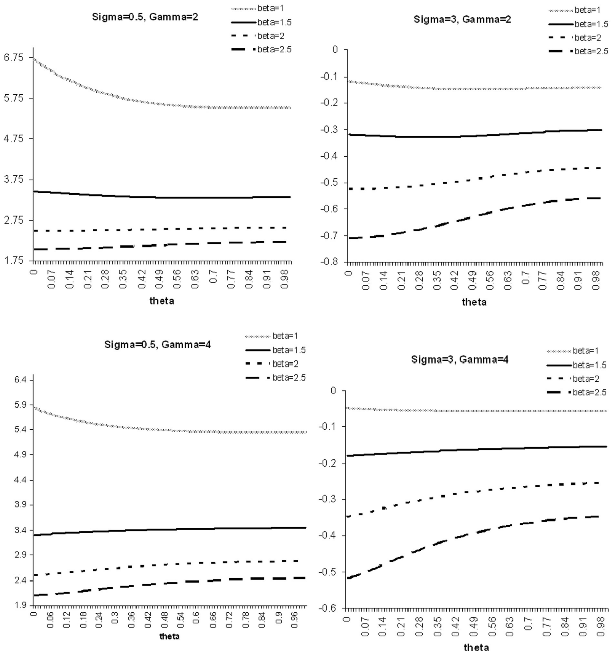
Fig. 1. Value functions.
