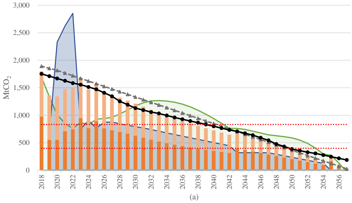
(a) — TNAC — MSR █ Final Auction █ Free Alloc -▲- Original cap ● Emissions ⋯ Thresholds
