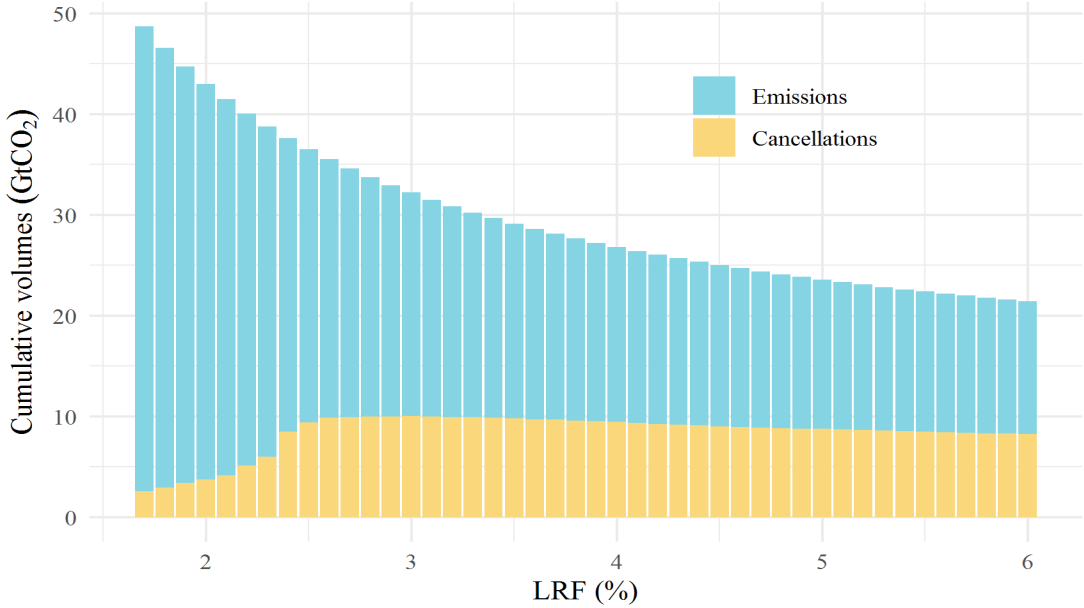
Figure 6. Impact of the LRF on certificate cancellations and cumulative 2020-2055 emissions.
