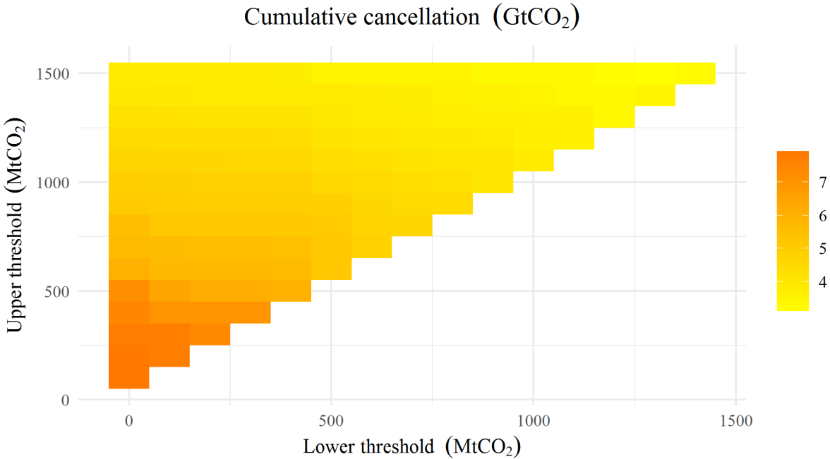
Figure 2. Impact of MSR thresholds on certificate cancellation.
