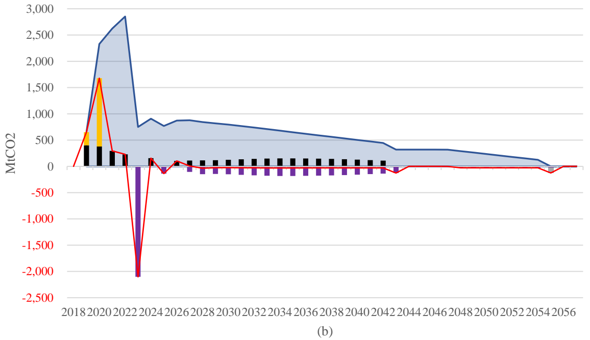
(b) — MSR █ Intake █ Cancellation █ Outtake █ Extra-intake — Net change
