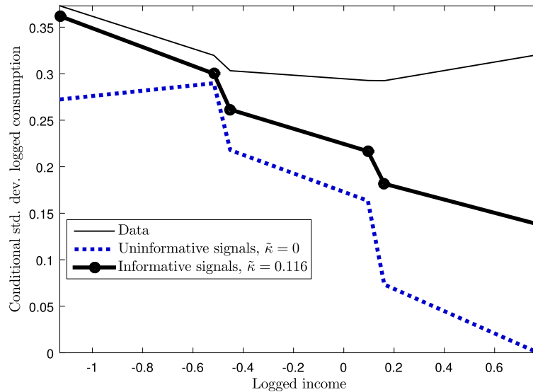
FIGURE 2. ESC model. Conditional standard deviation of logged consumption with respect to logged income for different precisions of the signals. The x -axis captures the logged income and the y -axis the conditional standard deviation of logged consumption. Income steps represent percentiles: [17th, 33th, 50th, 67th, 83th]. Solid line captures the conditional standard deviations for the years 1999–2003 in the CEX.
