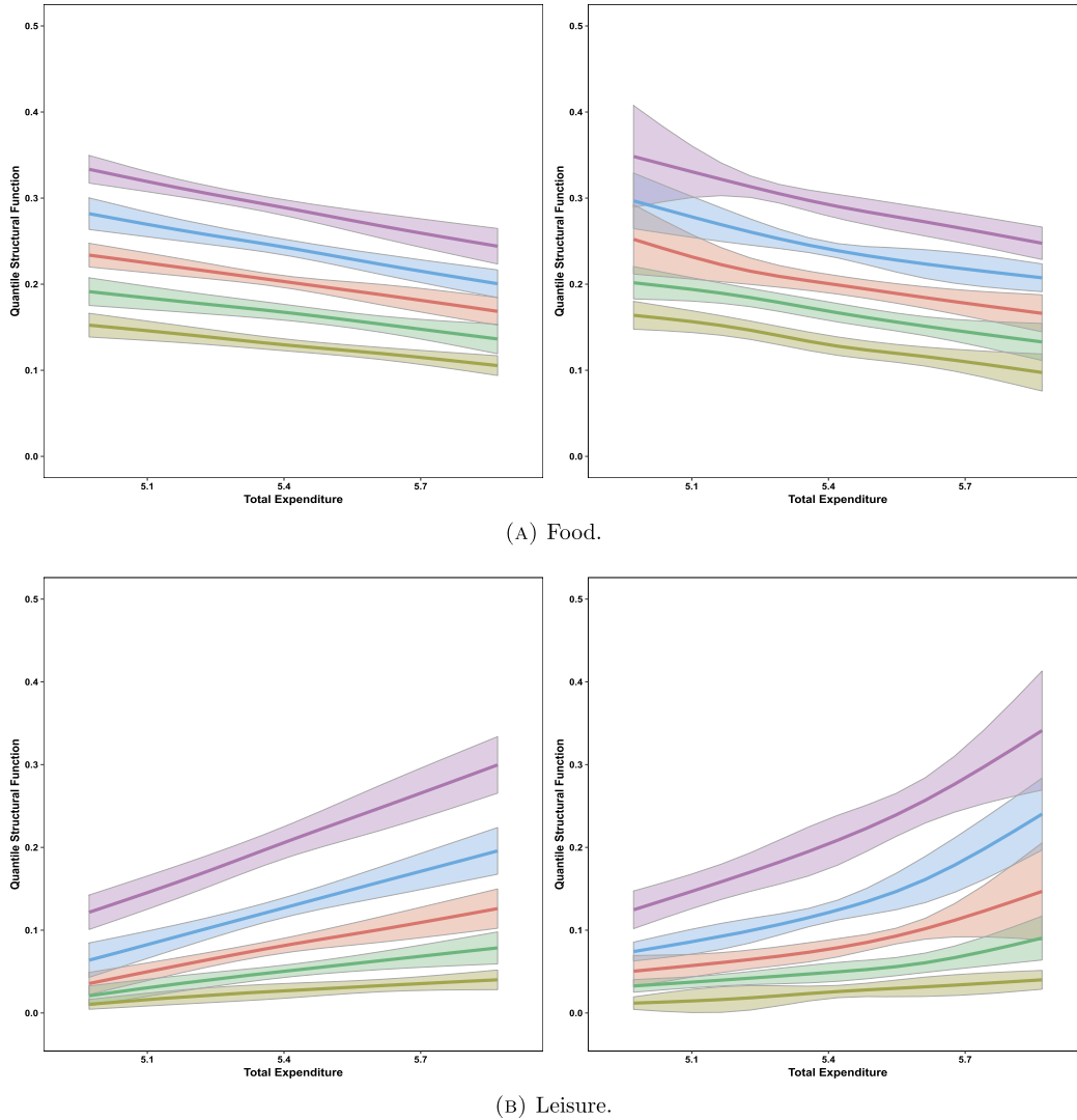
FIGURE D.4. QSF over \tilde{\mathcal{T}}_5 \tilde{\mathcal{A}}_5^* . Quantile (left) and distribution regression (right).
