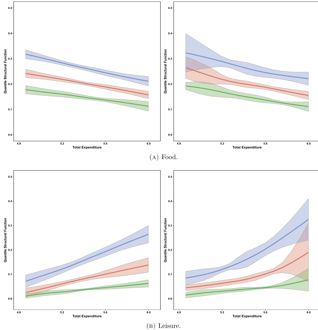
FIGURE D.2. QSF over \tilde{\mathcal{T}}_3, \tilde{\mathcal{X}}_7 . Quantile (left) and distribution regression (right).
