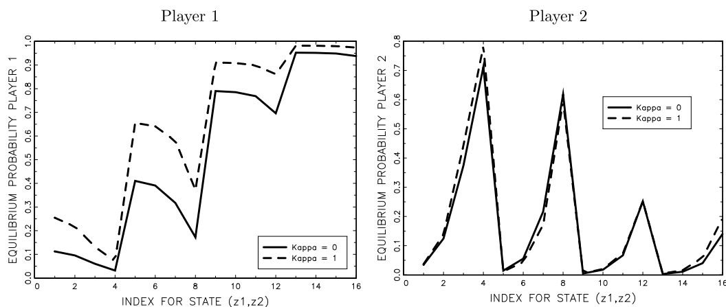
FIGURE 3. Equilibrium probabilities.
