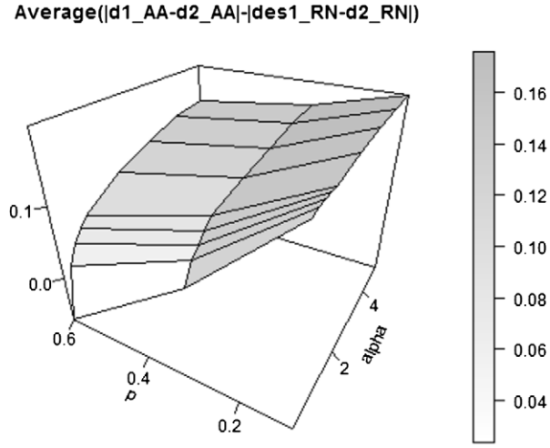
(a) Comparison of average distances between optimal maxmin and risk/ambiguity-neutral decisions, |d_1^{AA} - d_2^{AA}| - |d_1^{RN} - d_2^{RN}| for \gamma = \frac{1}{4} , different degrees of risk aversion \alpha , and different distribution parameters p . Each point corresponds to the average over (\nu_1, \nu_2) \in [-0.6, 0.6]^2 with a grid of size 0.05. The grid size for the decisions is 0.05, and the value of \epsilon = 0.4 .
