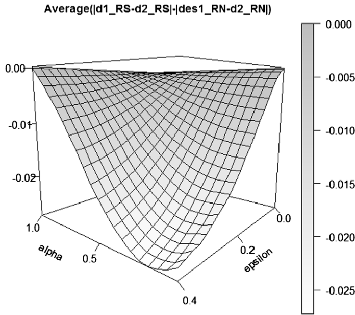
(b) Comparison of average distances between optimal risk-seeking and risk-neutral decisions, |d_1^{RS} - d_2^{RS}| - |d_1^{RN} - d_2^{RN}| for \gamma = \frac{3}{4} . Each point corresponds to the average over (\nu_1, \nu_2) \in [-0.6, 0.6]^2 with a grid of size 0.05. The grid size for \alpha is 0.05.
