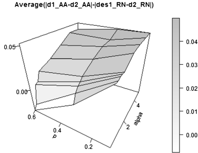
(b) Comparison of average distances between optimal maxmin and risk/ambiguity-neutral decisions, |d_1^{AA} - d_2^{AA}| - |d_1^{RN} - d_2^{RN}| for \gamma = \frac{3}{4} , different degrees of risk aversion \alpha , and different distribution parameters p . Each point corresponds to the average over (\nu_1, \nu_2) \in [-0.6, 0.6]^2 with a grid of size 0.05. The grid size for the decisions is 0.05, and the value of \epsilon = 0.4 .
