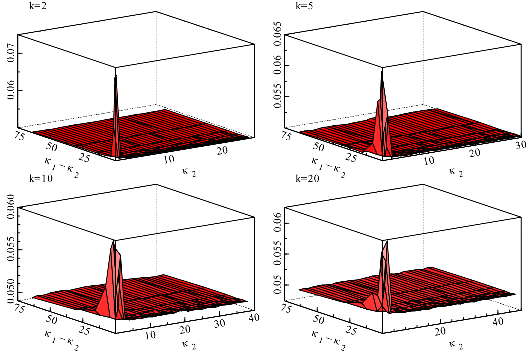
FIGURE 10. Size of the test \varphi_{\hat{A}^*} in step 5 of EMW's ALFD algorithm for each point under H_1 , \kappa_2 \in [0.1, \bar{\kappa}_2(k)] , \bar{\kappa}_2(2) = 25 , \bar{\kappa}_2(5) = 30 , \bar{\kappa}_2(10) = 38 , \bar{\kappa}_2(20) = 46 , discretized into 30 equally spaced points, and \kappa_1 - \kappa_2 \in \{0, 1, 2, 4, 8, 16, 32, 64\} . Calculated over 42 points of the nuisance parameter under H_0 , using 10,000 Monte Carlo replications with importance sampling.
