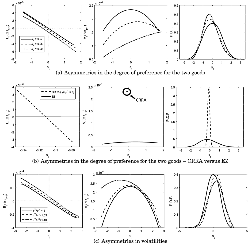
FIGURE 6. Asymmetric calibrations. Our model features Epstein and Zin (1989) preferences as specified in equation (14) and the endowments reported in equation (15). Our reference calibration is detailed in Section 5. We vary one parameter at a time, leaving the others unchanged.
