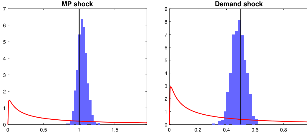
FIGURE C.2. Summary of posterior shock standard deviation ( \sigma ) draws for the bivariate SVMA model with prior smoothness \rho_{ij} = 0.9 . The plots show the true value (thick vertical line), prior density (curve), and histogram of posterior draws, for each \sigma_j , j = 1, 2 .
