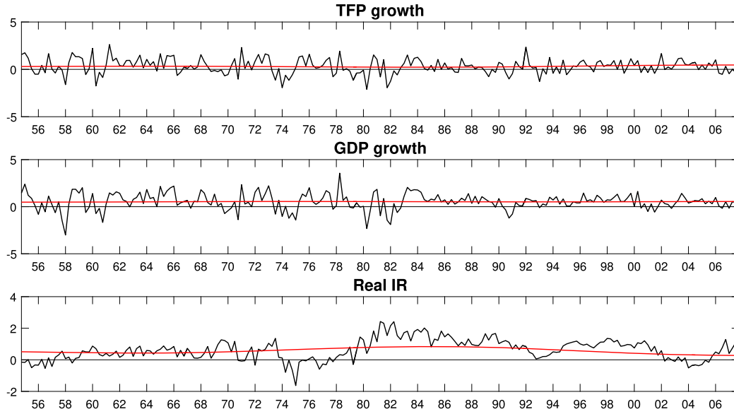
FIGURE C.14. Raw data on TFP growth, GDP growth, and the real interest rate (IR), along with estimated time-varying trends (smooth curves). The final data used in the empirical analysis are differences between the raw series and the trends.
