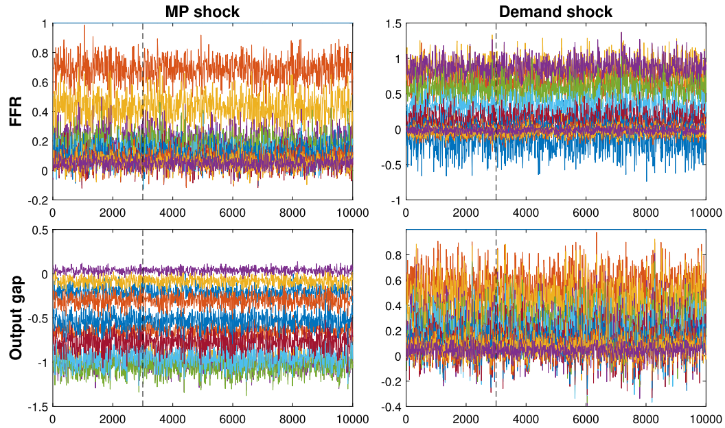
FIGURE C.10. MCMC chains for each IRF parameter ( \theta ) in the \rho_{ij} = 0.9 simulations in Section C.1.2. Each jagged line represents a different impulse response parameter (two of them are normalized at 1). The vertical dashed line marks the burn-in time, before which all draws are discarded. The horizontal axes are in units of MCMC steps, not stored draws (every 10th step is stored).
