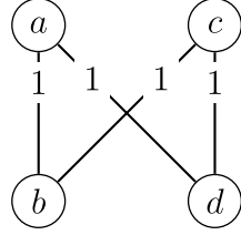
FIGURE 9. A four-player complete network with unit surplus.
