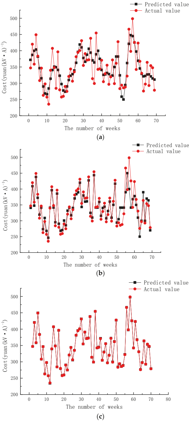
Figure 3. Prediction results. (a) The prediction result by EEMD-CS-SVM; (b) The prediction result by GCS-SVM; and (c) The prediction result by EEMD-GCS-SVM.
