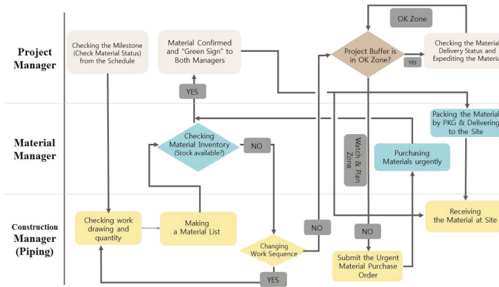
Figure 5. Flow Chart for Material Management Process.
