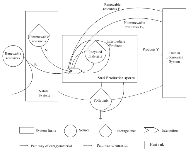
Figure 1. Material and energy flow diagram of the steel production process.
