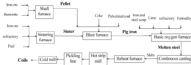
Figure 2. Flow diagram for the steel production process.
