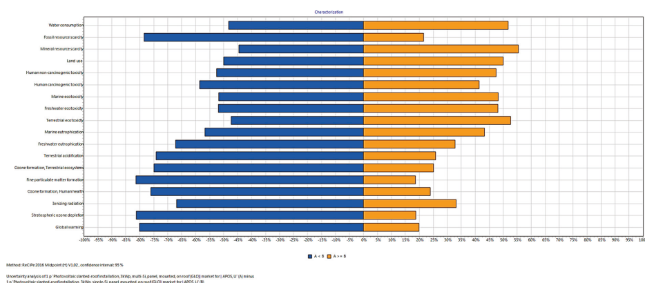
Figure 4. Monte-Carlo simulation results of LCIA uncertainties between mc-Si (A) and sc-Si (B) PV systems.
