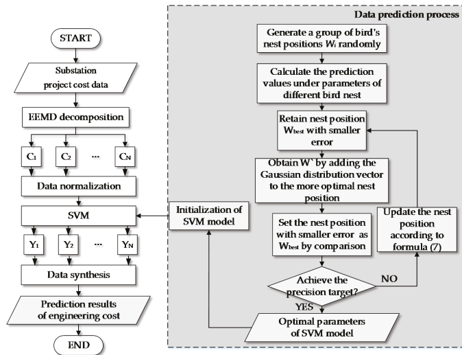
Figure 1. Flow chart of the Ensemble Empirical Mode Decomposition (EEMD)-GCS- Support Vector Machines (SVM) prediction model.
