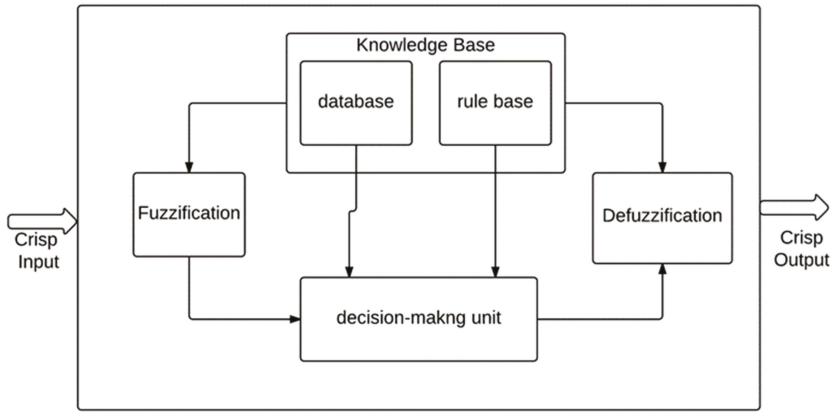
Figure 1. Fuzzy inference system (FIS). Adapted from [24].
