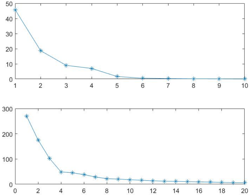
Figure 4: Scree plot of a system simulated by a S-DFM with N = 10 and T = 50 (top panel) and N = T = 100 (bottom panel).
