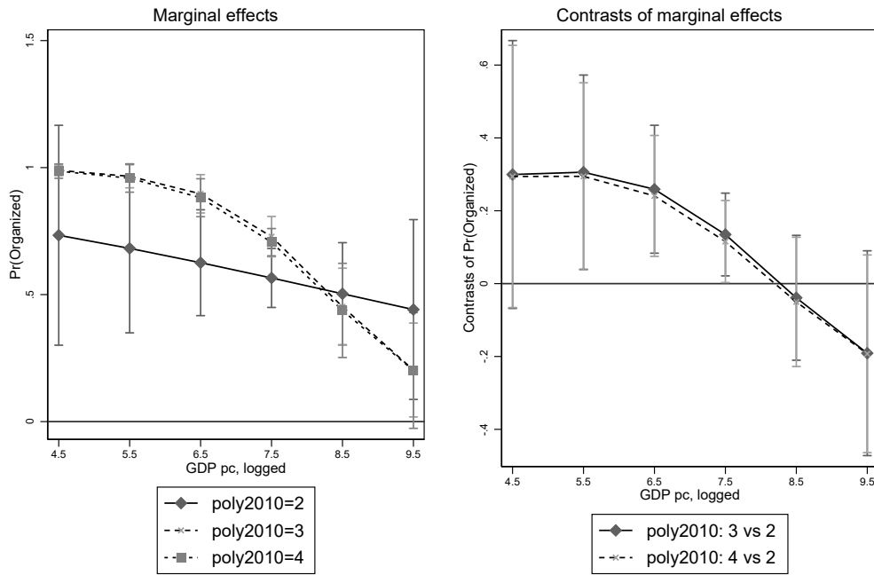
Figure 6: Organized social unrest: Polygyny and GDP interacted
