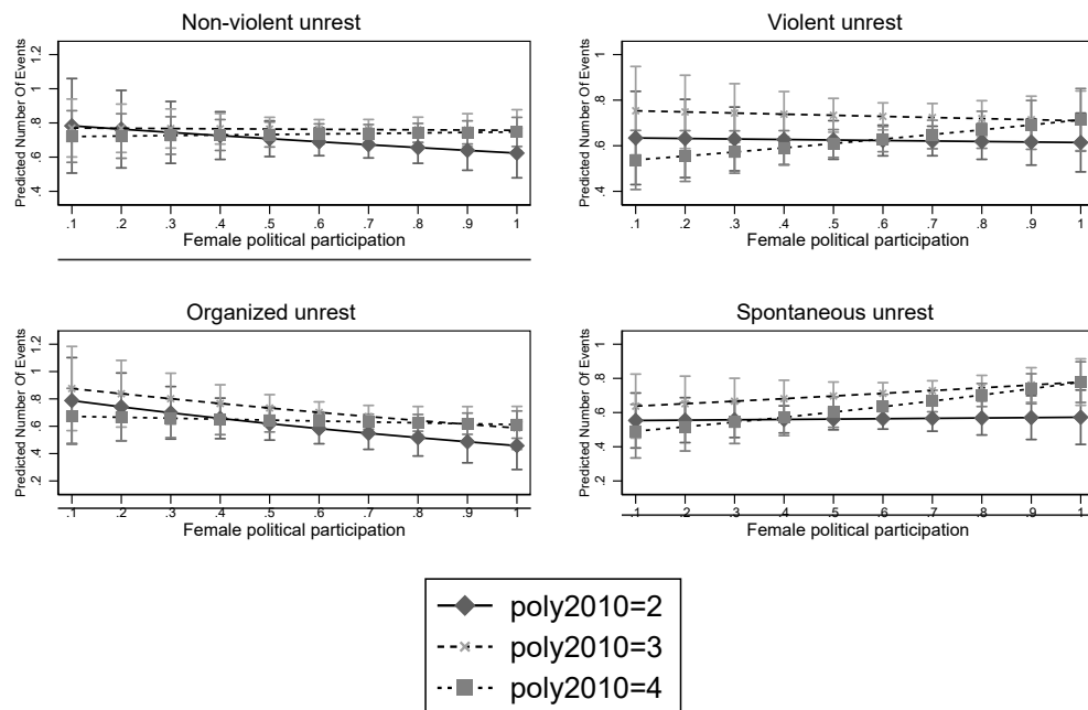
Figure B-5: Intensity: Interaction Effects for Female Political Participation and Polygyny
