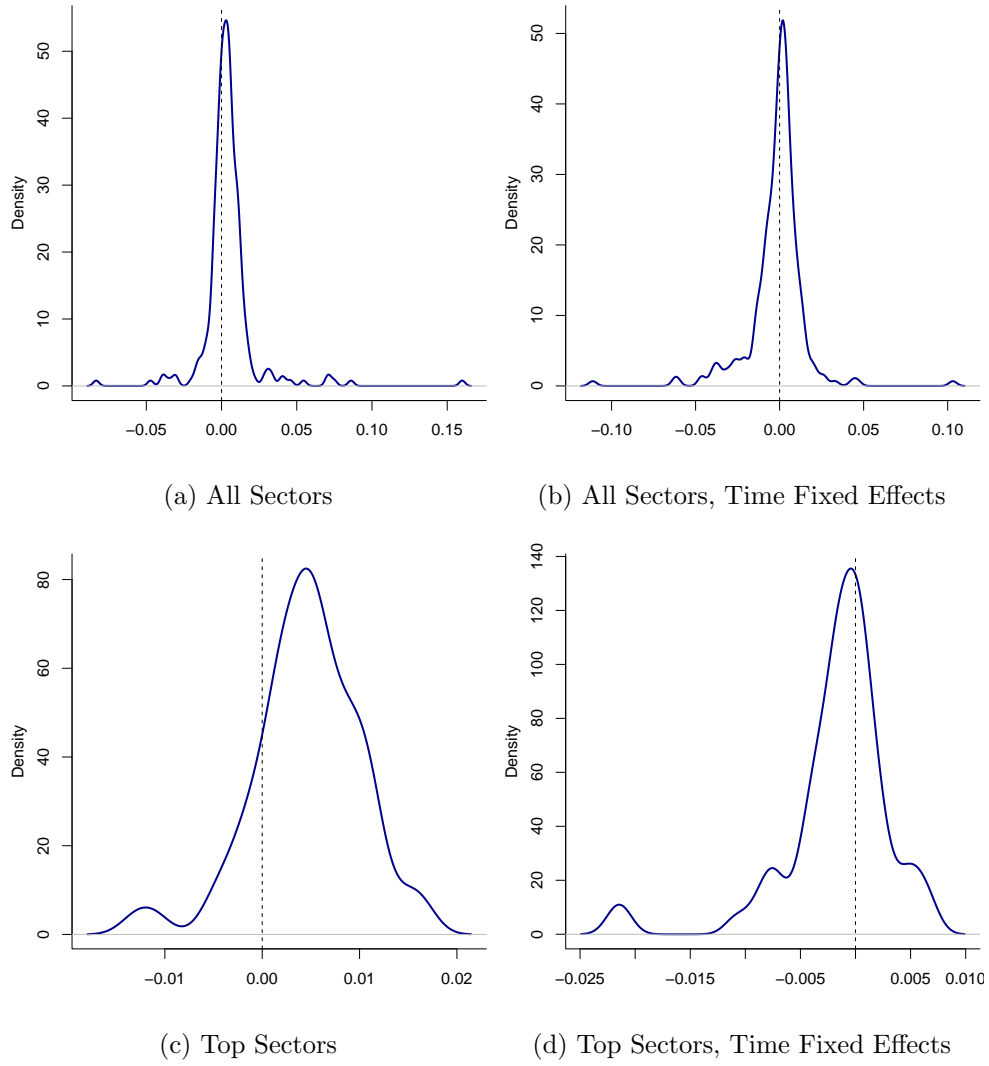
Figure A.13: Density of Error Term Covariances (Nominal)
