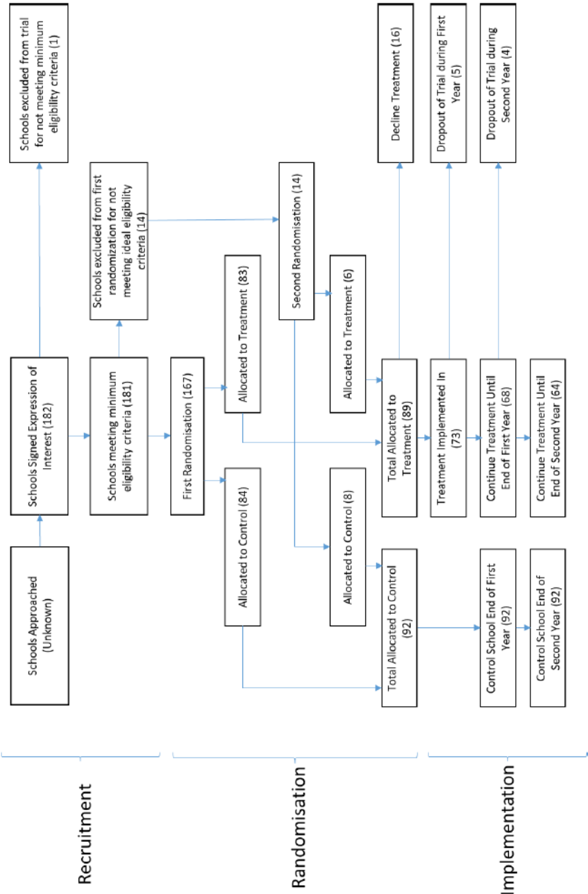
Figure 3: Consort flow diagram
