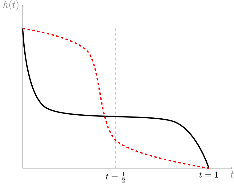
Figure 1: A function with a large \mathbb{V}[h(t)] (in red, dashed) and small \mathbb{V}[h(t)] (in black).
