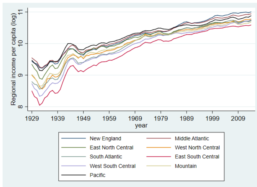
Figure A5: The logarithm of regional income per capita each year, between 1929 and 2014. The regional income per capita is adjusted for inflation and expressed in 2017US$. The nine US regions in the General Social Survey are defined in the "Material and Methods" section in the SI.
