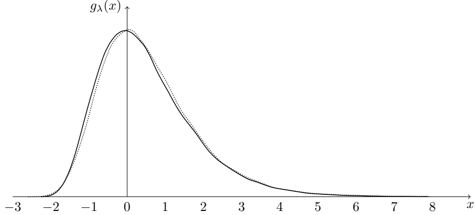
Figure 1: Approximate distribution for a C(\lambda) random variable
