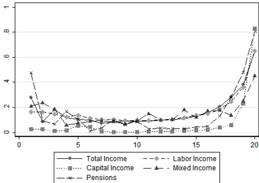
Figure 6: Persistence rates 2009-2016
