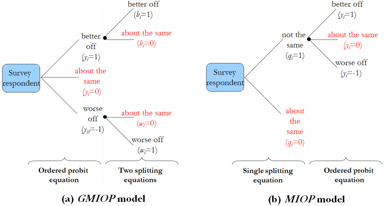
Figure 1: The Generalised Middle-Inflated Ordered Probit model ( GMIOP ) and its nested variant ( MIOP )
