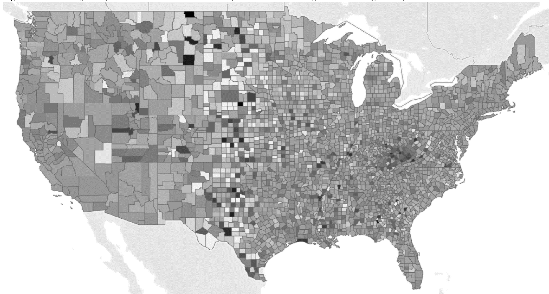
Figure A1.5: Rates of worry across US counties 2014–2016 (darker = more worry; white=missing values)
