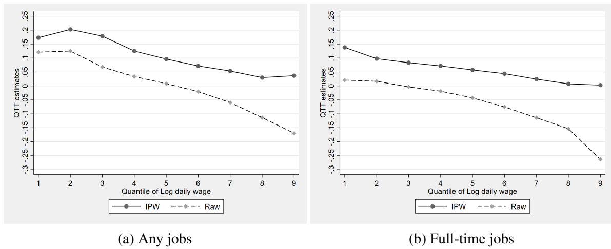
Figure A.1: QTT: before and after IPW weights
