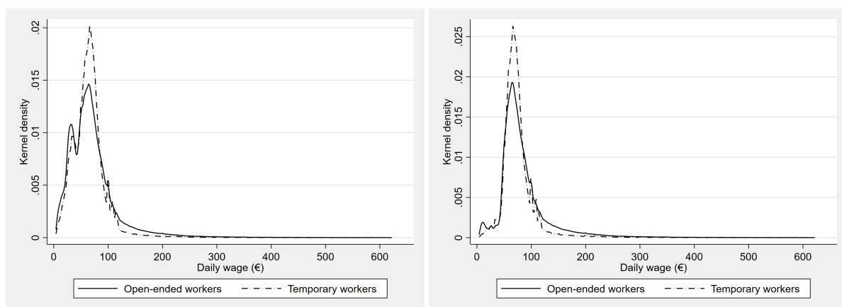
Figure 3: Kernel density estimates for daily wage by job contract
