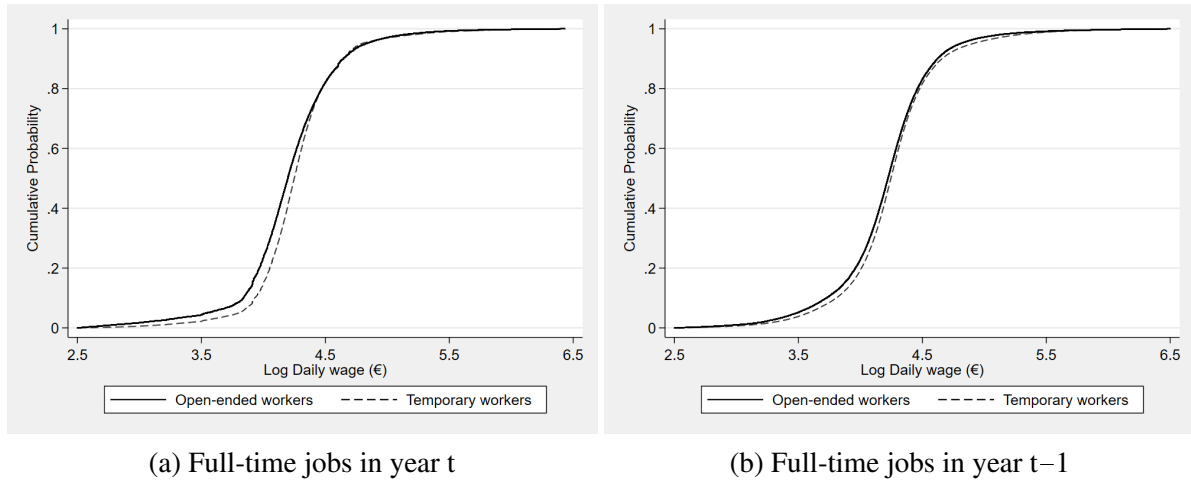
Figure A.4: Placebo test: cumulative distribution of daily wage logarithm—Full-time jobs
