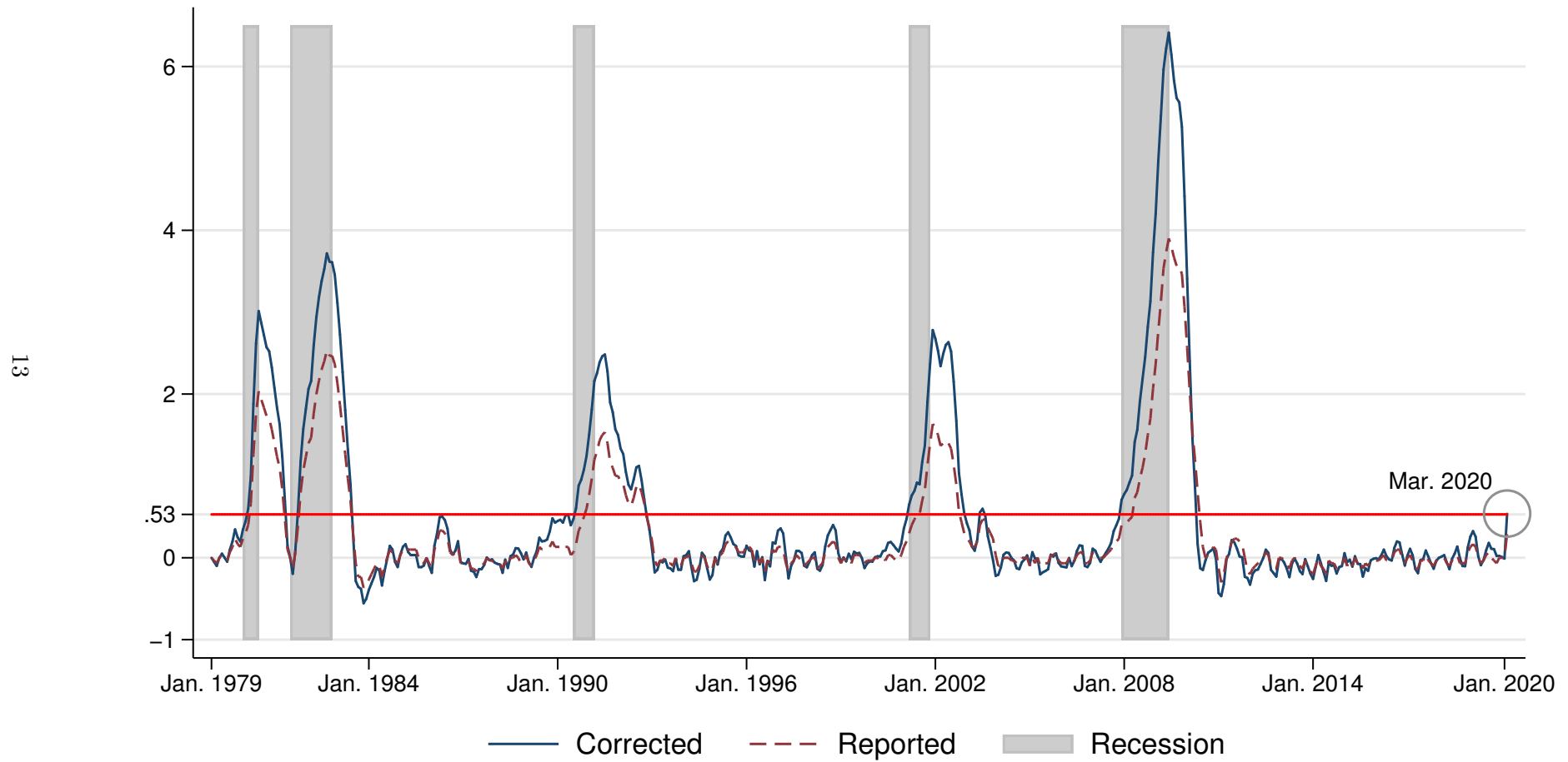
Figure 2: Real-time Sahm recession indicator: reported v.s. corrected
