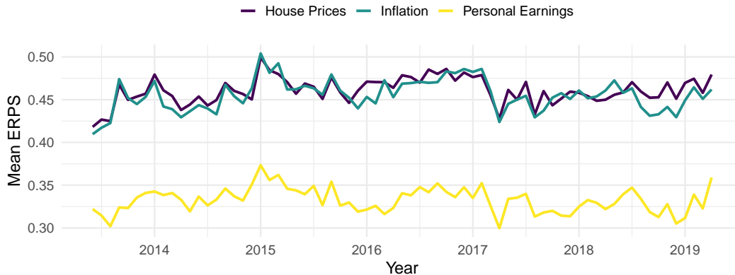
Figure 2: Mean ERPS for each month and variable.
