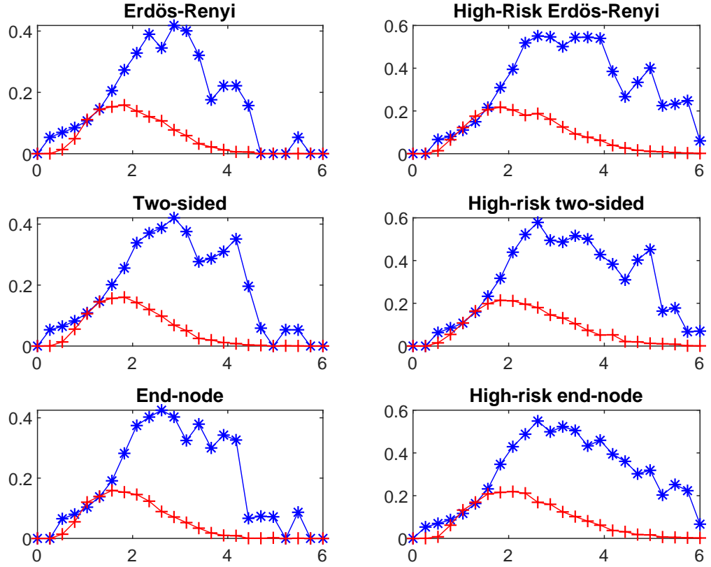
Figure 6: This graph shows the frequency and extent of contagion in the simulation of the model with Chinese characteristics. As before the curves with a star are the extent of contagion and the curves with crosses the frequency of a systemic crisis
