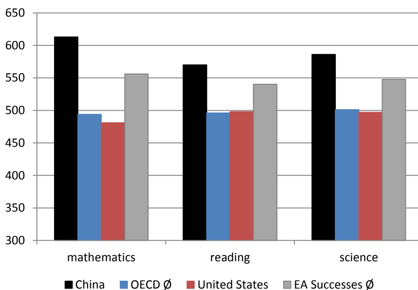
Figure 6. Pisa 2012 results.
