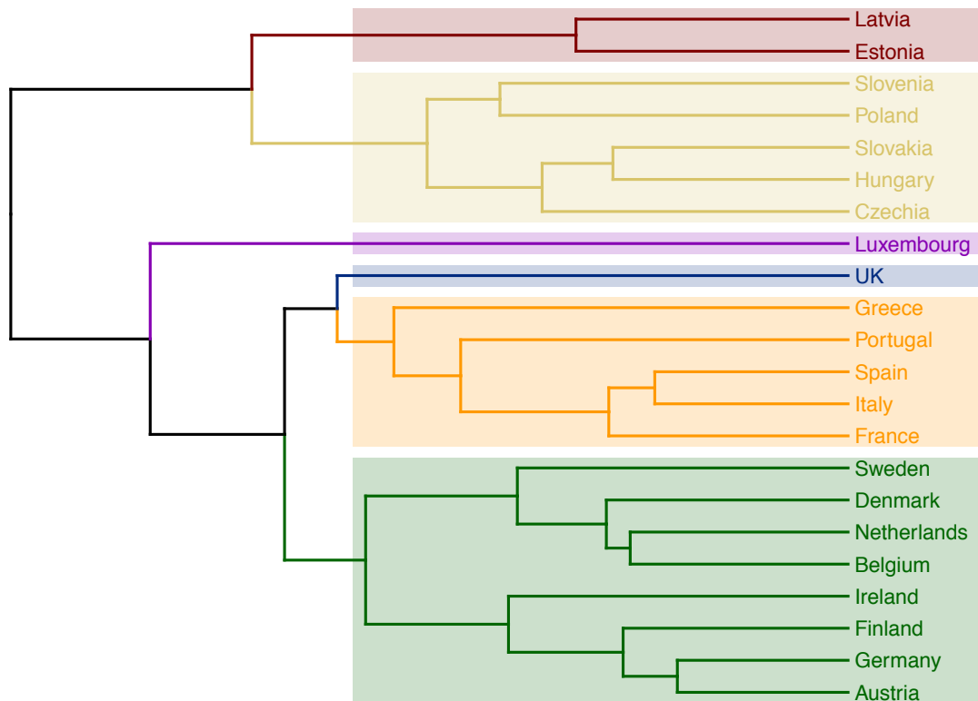
Cluster Dendrogram
