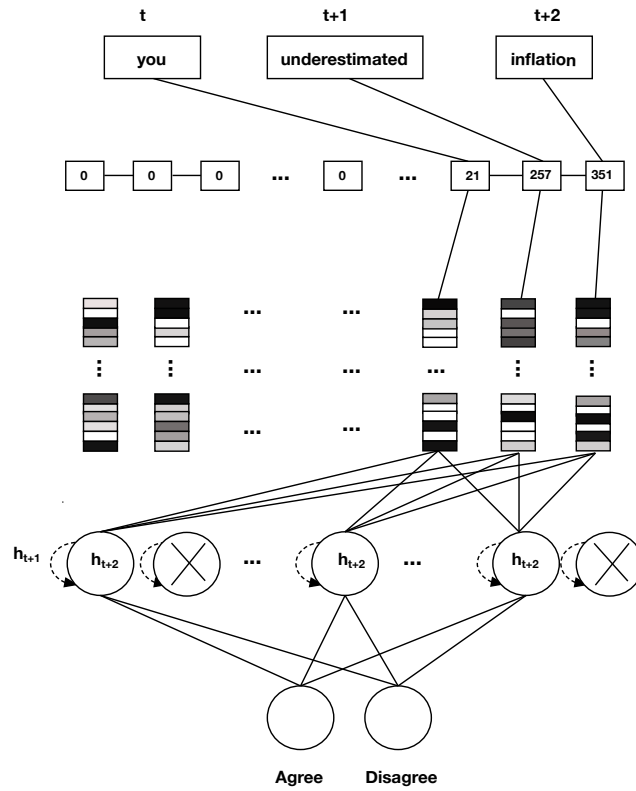
Figure 3: Long Short-Term Memory Model Architecture
