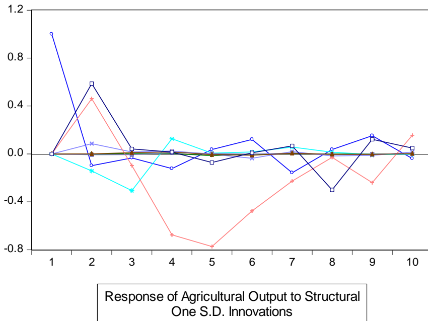
Figure 4: Response of Agricultural Output to Shocks in the Guided Deregulated regime (1987-2016)
