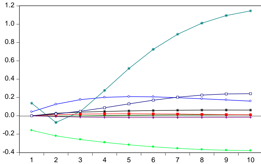
Response of Industrial Output to Structural One S.D. Innovations
