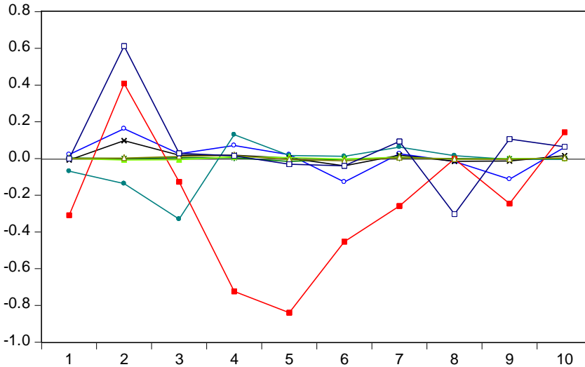
Figure 5: Response of Industrial Output to Shocks in the Regulated Regime (1961-1986)
