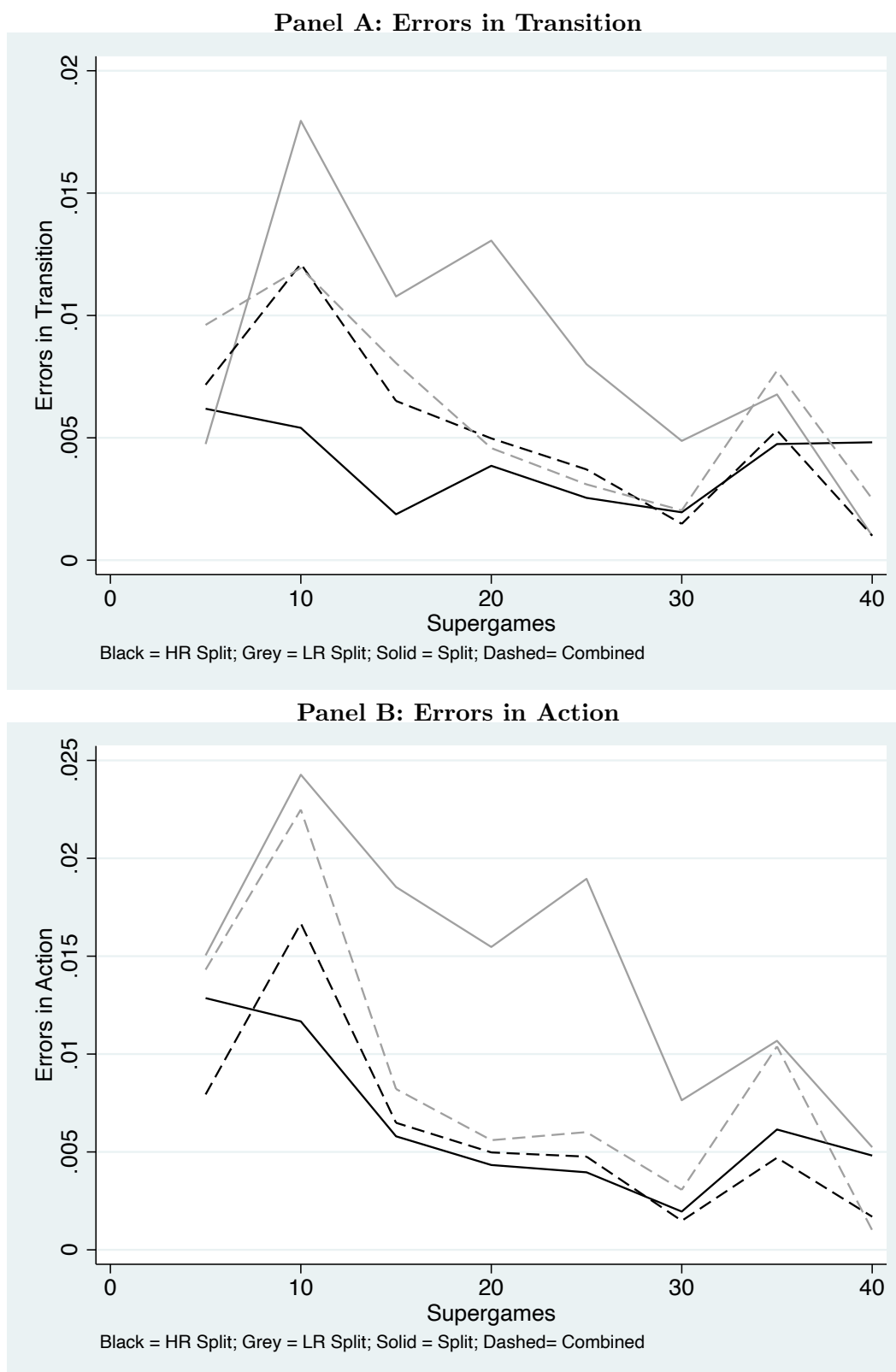
Figure A.3: Errors in transition and action , Error rates across different treatments and groups. The average is computed over observations in successive blocks of five supergames. The grey solid line represent the low-IQ split treatment, the black solid lines the high-IQ split treatment, the dashed lines the combined treatment: grey is the low-IQ group, black is the high-IQ group.
