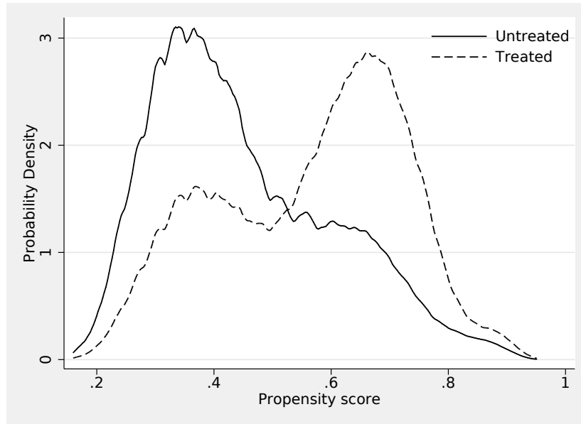
Figure 2: Distribution of the propensity score, with year fixed-effects (without university/period fixed-effects).
