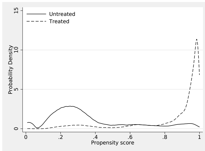
Figure 1: Distribution of the propensity score in the treated and non-treated group
